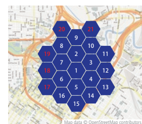
12.5 kHz digital system At a total of 2150 sq. miles coverage: 5.8-mile radius per site / 21 site total
